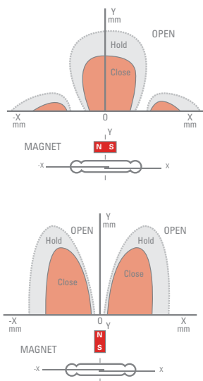
Figure 2—Single-pole linear activation, perpendicular orientation
